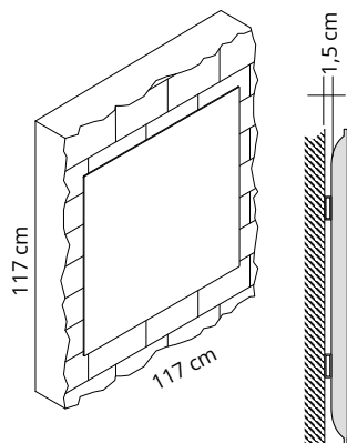
Dettaglio attacchi magnetici (inclusi) Connections of magnetic detail (included)
